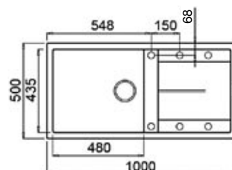
UNICO 480 cm. 100x50 (1 v. prof. 20) (foro incasso 98x48)
