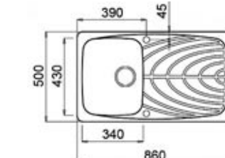
MASTER 400 cm. 86x50 (1 v. prof. 22) (foro incasso 84x48)
