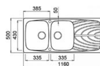
MASTER 500 cm. 116x50 (2 v. prof. 22) (foro incasso 114x48)
