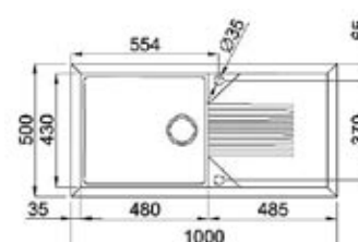
TEKNO 480 cm. 100x50 (1 v. prof. 22,5) (foro incasso 98x49)
