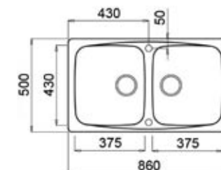
MASTER 450 cm. 86x50 (2 v. prof. 22) (foro incasso 84x48)
