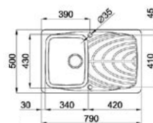
MASTER 300 cm. 79x50 (1 v. prof. 22) (foro incasso 77x48)
