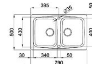
MASTER 350 cm. 79x50 (2 v. prof. 22) (foro incasso 77x48)
