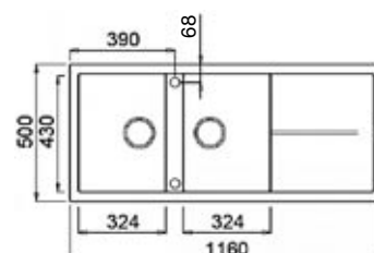
UNICO 500 cm. 116x50 (2 v. prof. 20) (foro incasso 114x48)
