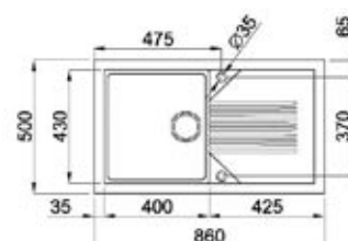
TEKNO 400 cm. 86x50 (1 v. prof. 22,5) (foro incasso 84x48)
