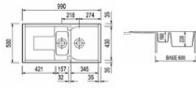
CORAX CX0991 cm. 99x50 1 v. e 1/2 Prof. 23/16 - (foro incasso 97x48)
